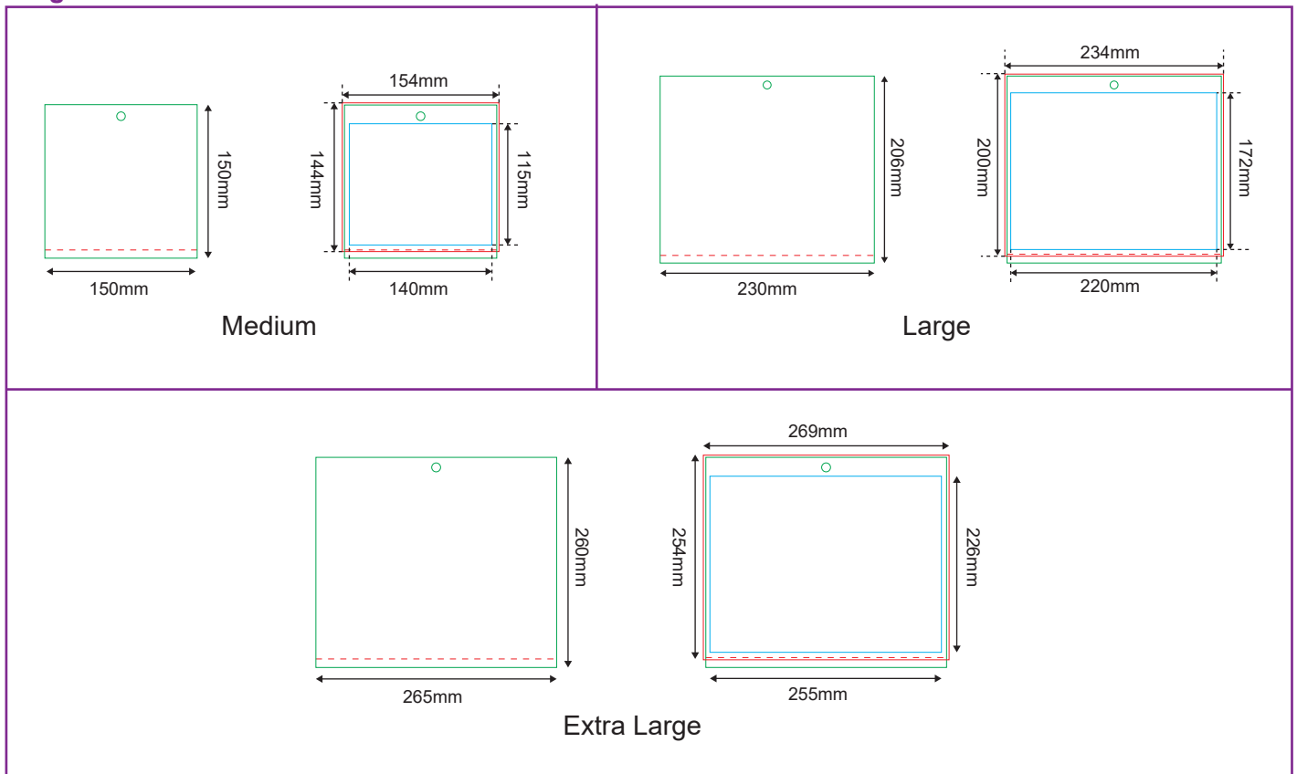
Diagram shows Header's Artwork Dimension :
